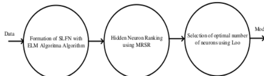
Fig.3. Fig. The three main steps of the ELM Method
