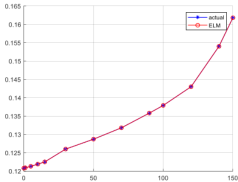
Fig. 8 Voltage Collapse Prediction Using ELM for Bus 41 (Bus Pangkep)
