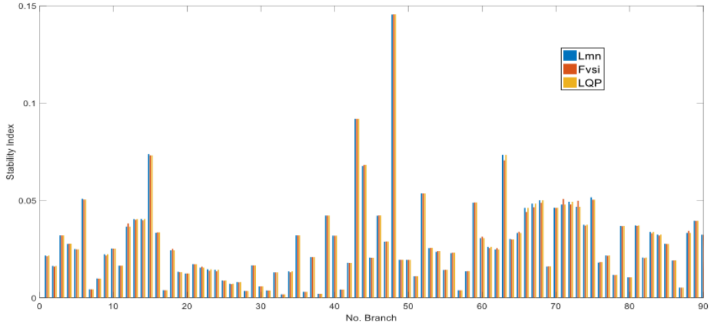
Fig. 6 Comparison of Voltage Stability Index Values in the South Sulawesi Electrical System
