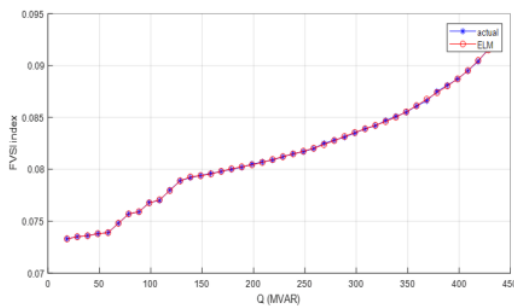
Fig. 9 Voltage Collapse Prediction Using ELM for Bus 11 (Bus Bulukumba)
